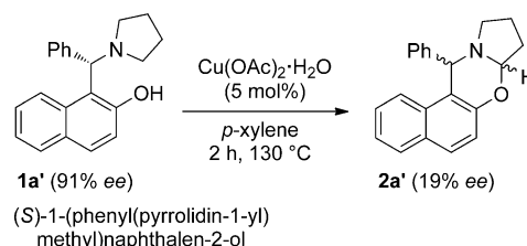
Scheme 4. Reaction using chiral substrate.
