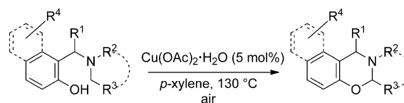
Scheme 1. Synthesis of 2,3-dihydro-1,3-oxazines.
