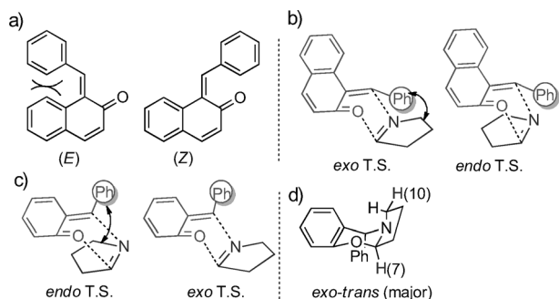
Figure 1. a) Steric repulsion destabilizes the E form. b) Steric repulsion in the exo transition state. c) Steric repulsion in the endo transition state. d) W coupling. T.S. = transition state.
