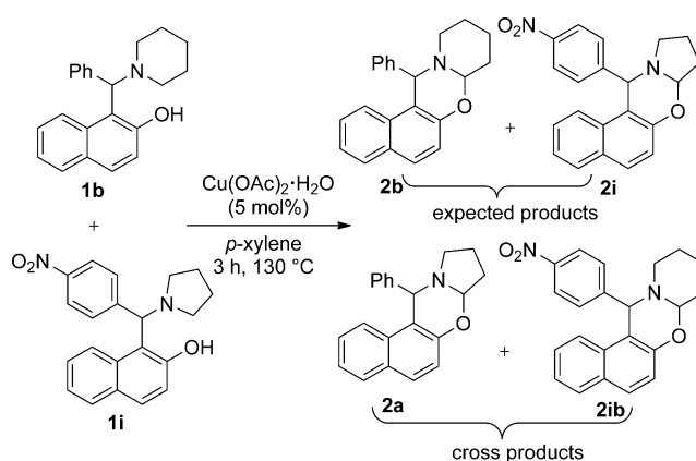
Scheme 3. Cross reaction between two substrates furnishing four products.
